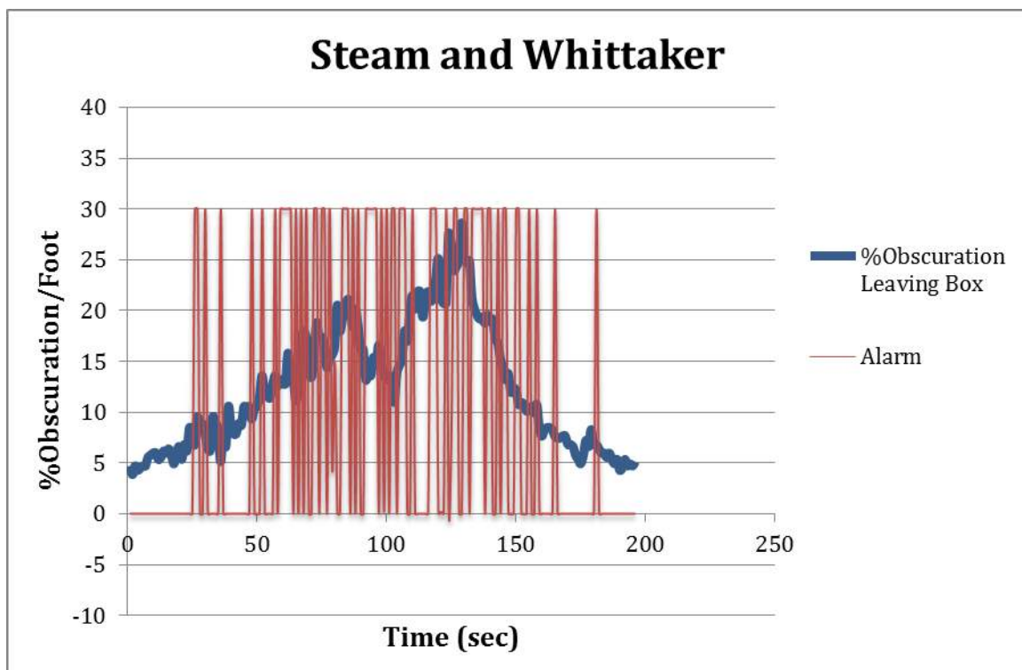
Figure 33 – Water Steam Alarming Whittaker Detector at Different Percent Obscurations
