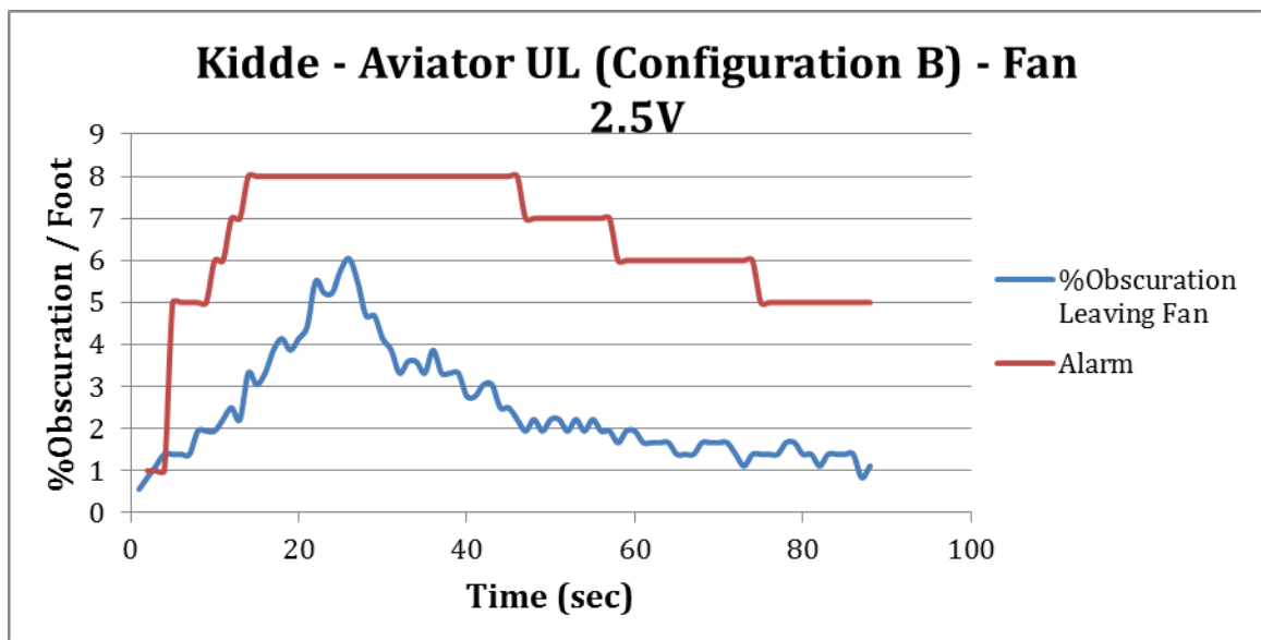
Figure 28 – Percent Obscuration Testing of Kidde Detector with Aviator UL Smoke machine with 2.5V Fan
