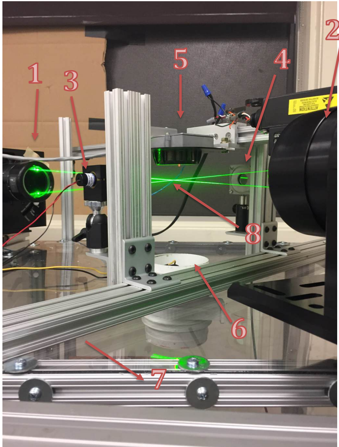
Figure 11 - Equipment Above Testing Chamber Including: PDPA Laser(1) and its Receiver (2), Optical Density Laser (3) and its Receiver (4), Kidde Detector in Alarm (5), Exit Fan (6) on top of Testing Chamber (7), and the Measurement Point (8)
