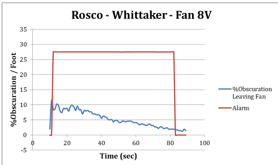
Figure 26 –Data for Whittaker Detector Going “Into Alarm” with Rosco Smoke Machine with 8V Fan
