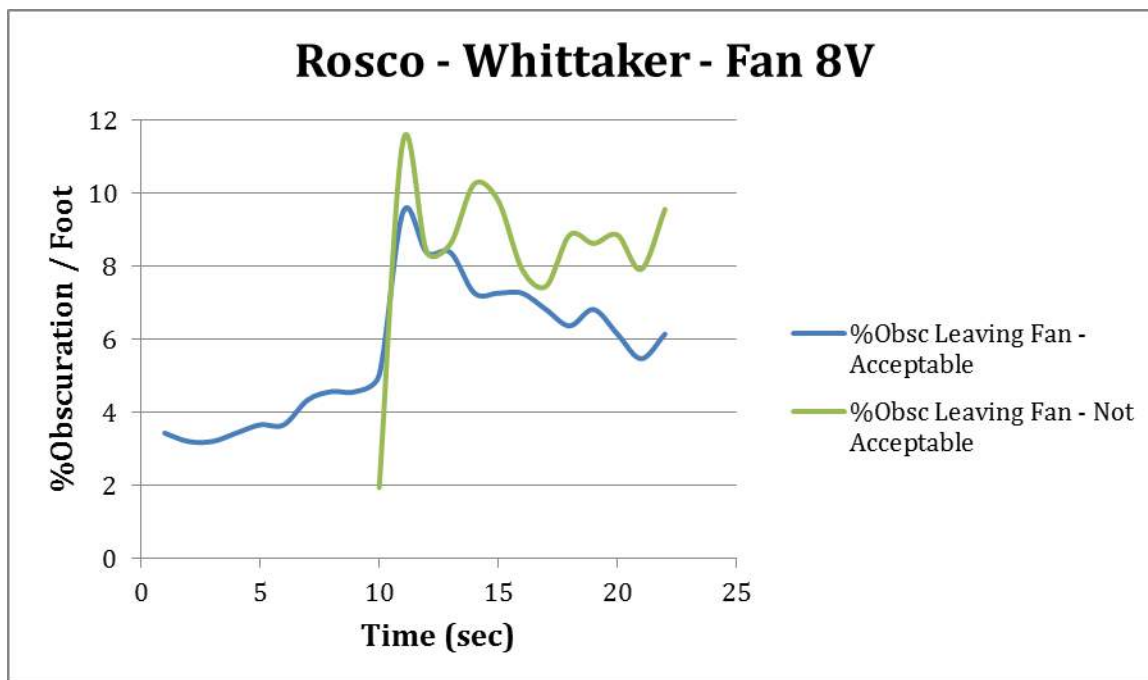
Figure 27 – Comparing Runs ‘April5 001’ and ‘April5 007’ introduction of peaks for two different runs with Rosco Smoke Machine and Whittaker detector
